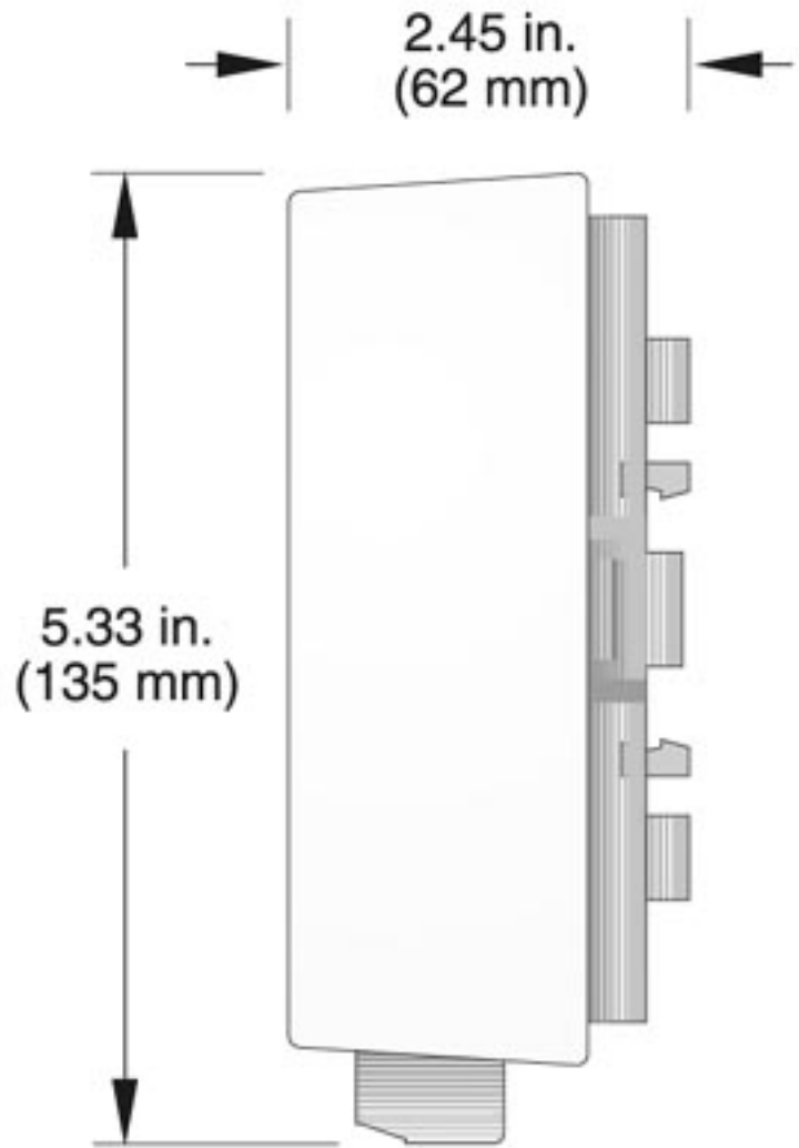
Dimensioned drawing
