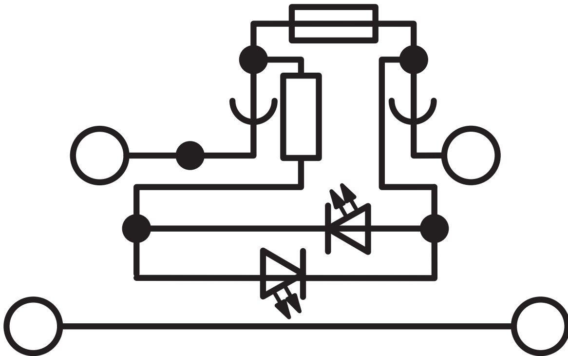
Circuit diagram
