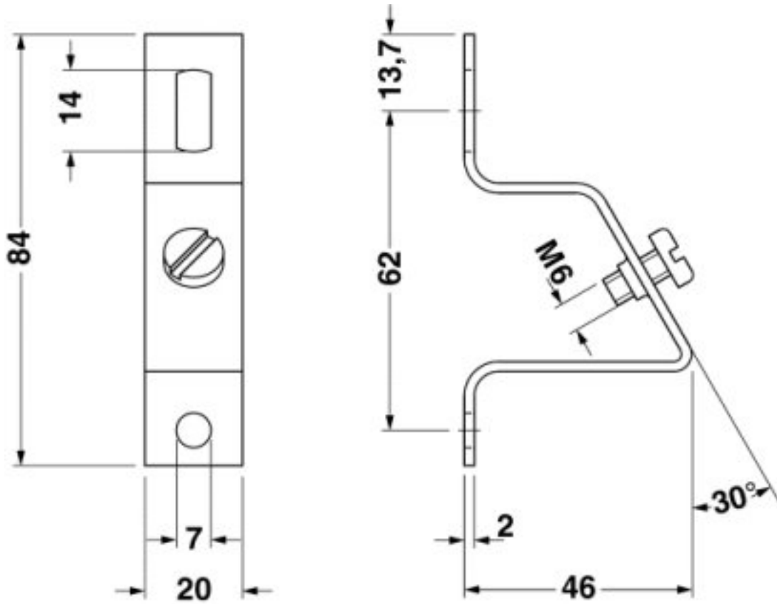
Dimensioned drawing
